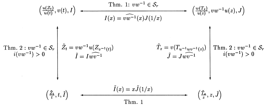
FIG. 1. Commutative diagram relating LDPs, based on Theorems 1 and 2.
