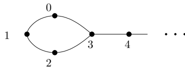
Figure 1: The graph defined in the Remark 3.3.
