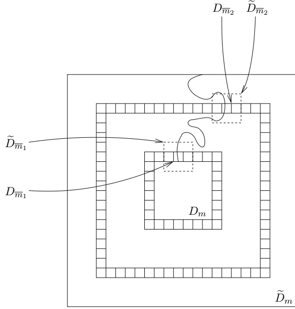
Figure 2: The figure shows all the boxes with indexes in \mathcal{K}_1 and \mathcal{K}_2 . Note that the event B_m^u implies B_{\bar{m}_1}^u and B_{\bar{m}_2}^u for some \bar{m}_1 \in \mathcal{K}_1 and \bar{m}_2 \in \mathcal{K}_2 .
