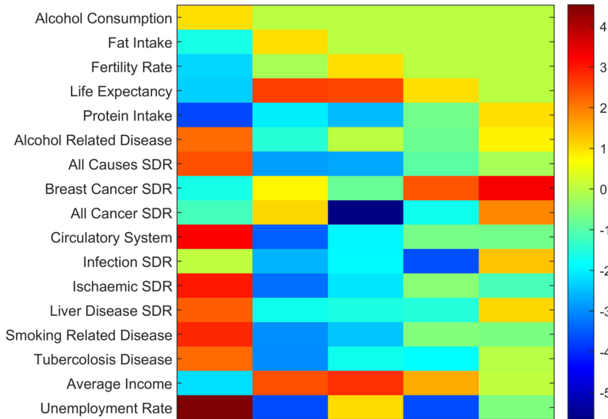
Figure 9: Factor Loadings.
