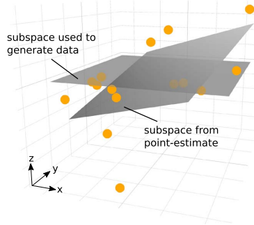
Figure 8: Three dimensional data generated from (5.1) with p = 2, W = I_{3,2}, \Lambda_{11} = 2, \Lambda_{22} = 1 and \sigma = 1 . The maximum-a-posteriori (MAP) estimate of PPCA corresponds to a single orthogonal matrix in the Stiefel Manifold that is closest, in terms of average squared distance, to the set of points. When there are few data points relative to the size of the matrix, this point estimate can often have high variance.
