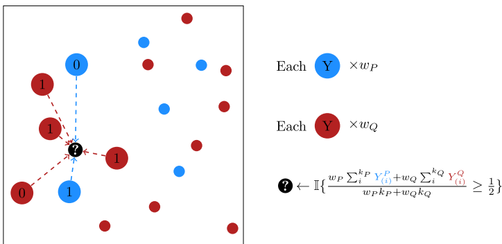
FIG. 2. An illustration of the two-sample weighted K -NN classifier. (X^P, Y^P) are shown by the blue points and (X^Q, Y^Q) are shown by the red points. For each point in the graph, the coordinates represent its two-dimensional covariates X while the number marked inside the point represents its label Y . To classify the black point ( x ) located in middle of the graph, by calculation we get (say) k_P = 2 and k_Q = 4 . Then we find k_P nearest neighbors from P -data and k_Q nearest neighbors from Q -data. Finally, we calculate their weighted mean to make the final classification.
