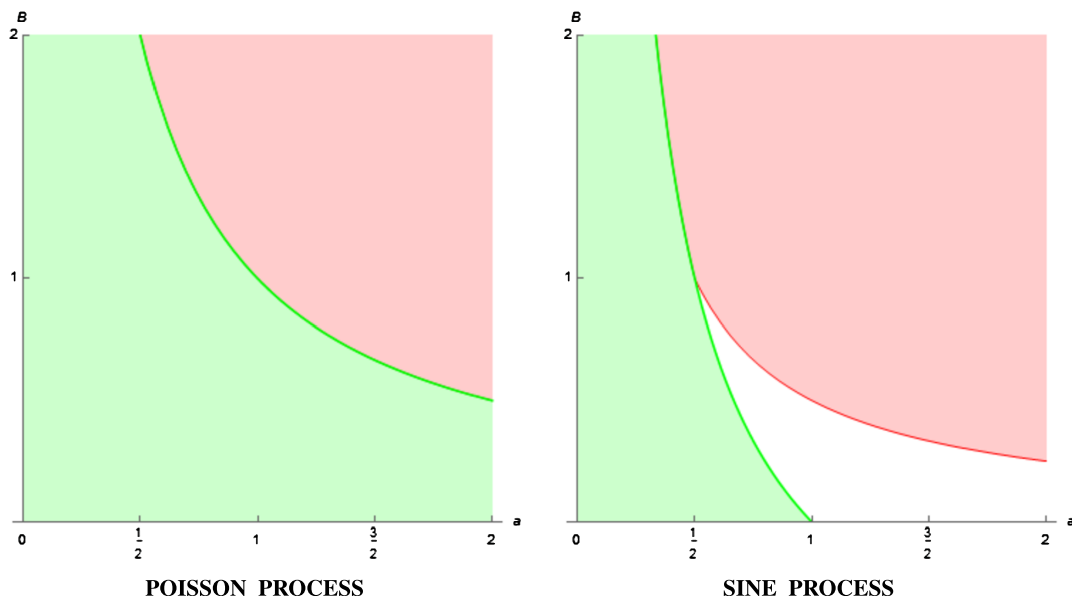
FIG. 1. A plot of the regions (a, B) for which the Poisson process and sine process can be mimicked at bandwidth B by a point process with uniform moments supported on a\mathbb{Z} . In the green region these point processes can be mimicked, while in the red region they cannot. In the white region of the second plot we currently have no information.
