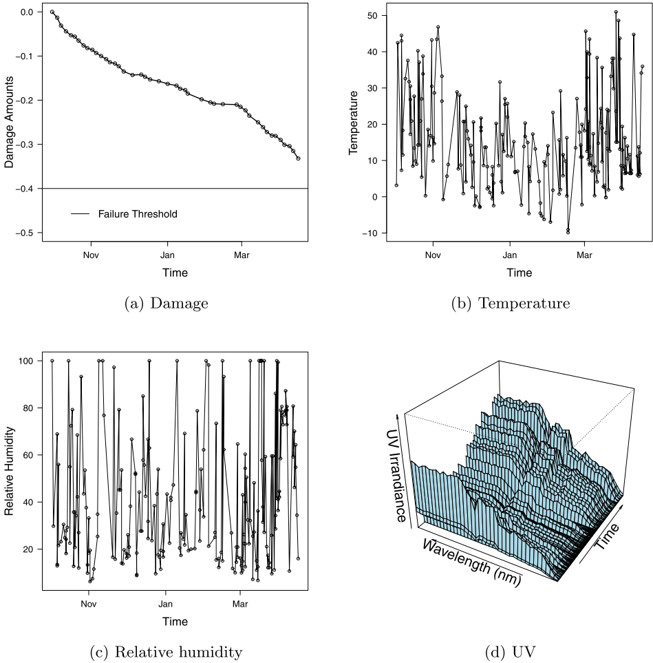
FIG. 6. Plots of the degradation path for an outdoor-exposed specimen showing the relationship between the degradation and the dynamic covariates. (a) The degradation path, (b) temperature as a function of time, (c) RH as a function of time, and (d) a perspective plot showing the recorded UV intensity as a function of time and wavelength.
