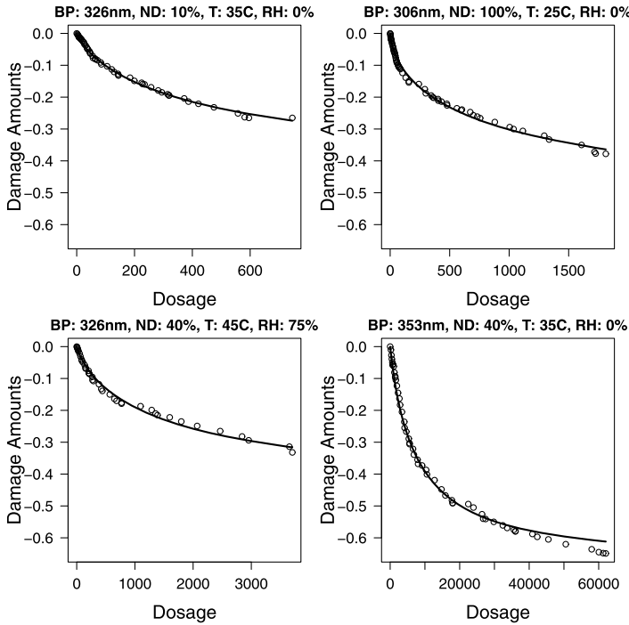
FIG. 8. Fitted degradation paths for four randomly selected specimens based on the model in (11). The points are the measured values and the lines show the fitted values. The plot titles show the levels of the experimental factors.
