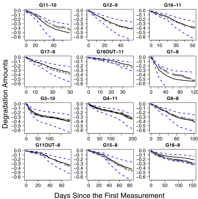
FIG. 9. Prediction results for 12 representative outdoor-exposed specimens. The points show the measured values, the solid lines show the predicted values, and the dashed lines show the 95% point-wise prediction intervals.
