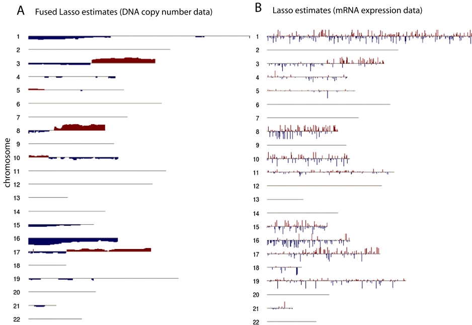
FIG. 7. Penalized coefficient vector estimates arranged by chromosomes 1 to 22 derived by iCluster (fused lasso, lasso) applied to the Chitale et al. lung cancer data set. A single latent variable vector is used to identify the major pattern of each chromosome.
