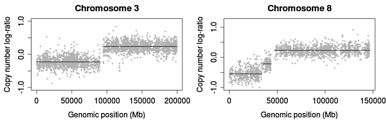
FIG. 6. Illustration of copy number probe-level data from a lung tumor sample [Chitale et al. (2009)]. Log-ratios of copy number (tumor versus normal) on chromosomes 3 and 8 are displayed. Log-ratio greater than zero indicates copy number gain and log-ratio below zero indicates loss. Black line indicates the segmented value using the circular binary segmentation method [Olshen et al. (2004), Venkatraman and Olshen (2007)].
