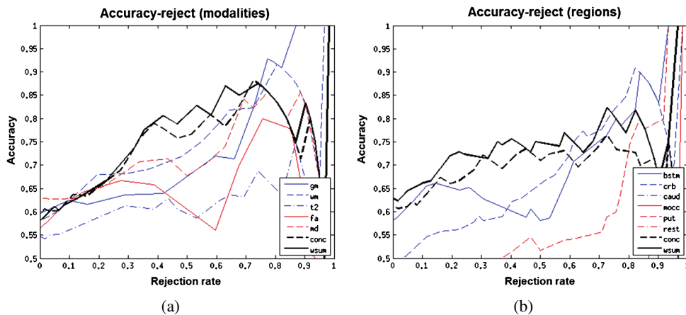
FIG. 5. (a) Accuracy–reject curve for multi-modality classifiers. (b) Accuracy–reject curve for multi-region classifiers.
