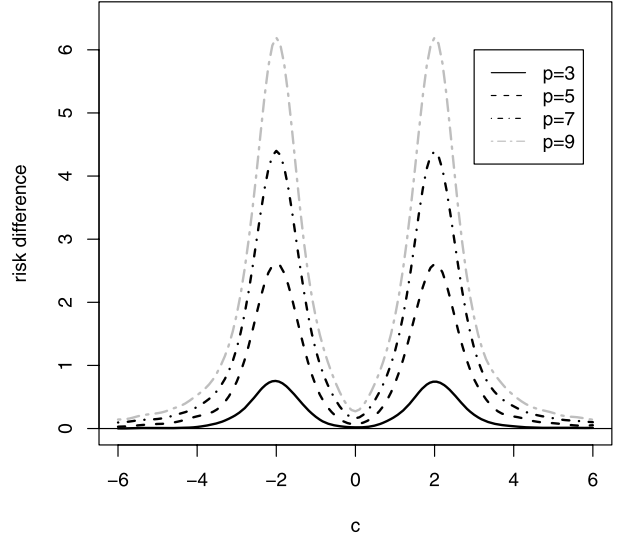
FIG. 3. The risk difference between \hat{p}_U and multiple shrinkage \hat{p}_{H^*} when \mu = (c, \dots, c)' , v_x = 1 , v_y = 0.2 , b_1 = (2, \dots, 2)' , b_2 = (-2, \dots, -2)' , and w_1 = w_2 = 0.5 .
