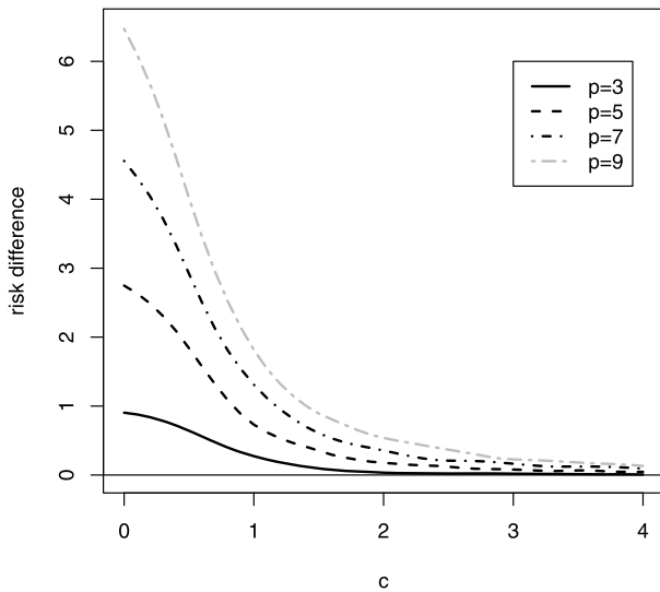
FIG. 2. The risk difference between \hat{p}_U and \hat{p}_H when \mu = (c, \dots, c)' , v_x = 1 , v_y = 0.2 .
