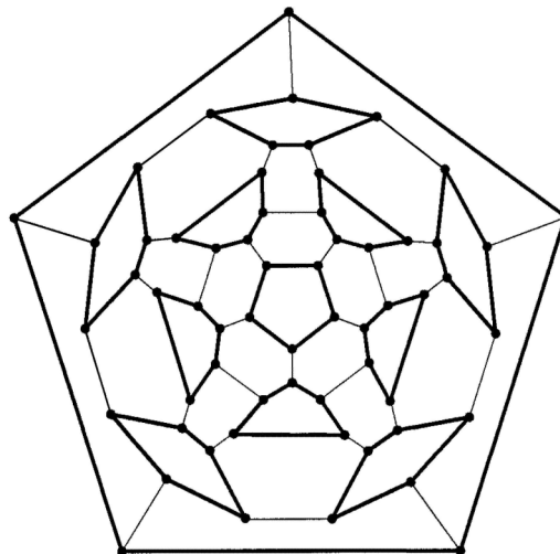
Fig. 3. A preparatory graph G' to get a planar graph G with M^*(G) = 4 and with no cycles of length from 4 to 8.
