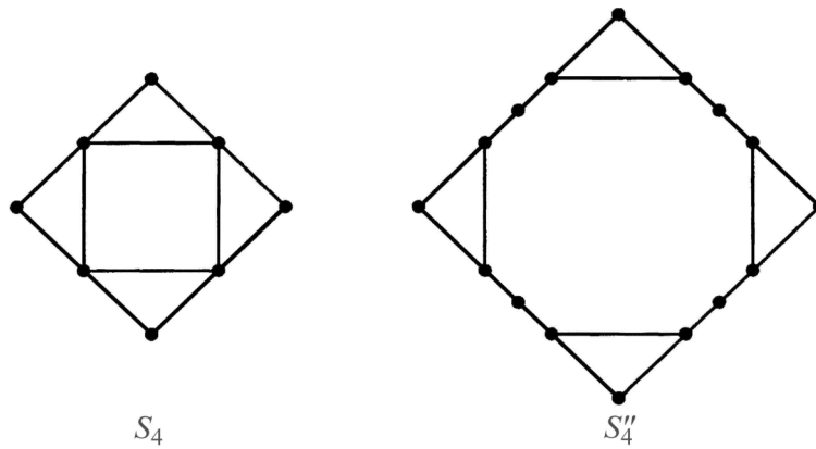
Fig. 1. Sunflower S_4 on the left and split sunflower S_4'' on the right.
