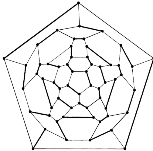
Fig. 2. A preparatory graph G' to get a planar graph G with M^*(G) = 5 and with no cycles of length from 4 to 6.
