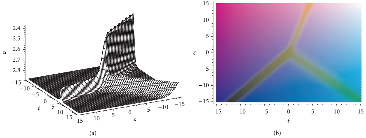
FIGURE 1: Plot of the interaction solution between one soliton and one resonant soliton solution for field u with the parameters k = 1/2, b = 1, k_0 = 1/4, l_0 = 1/4, b_0 = 1/2, and \omega_0 = 1/2 . (a) Three-dimensional image at x = y = 0 . (b) The density plot of the corresponding solution.
