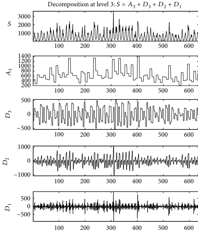
FIGURE 4: Decomposed wavelet subtime series components ( D_s ) of runoff data of Tangnaihai station.
