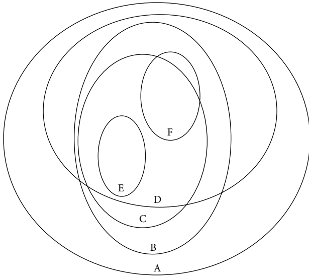
FIGURE 1: Inclusion relationships among classes of completely monotonic and related functions on (0, \infty) . (A) Almost completely monotonic function class. (B) Completely monotonic function class. (C) Logarithmically completely monotonic function class. (D) Almost strongly completely monotonic function class. (E) Strongly logarithmically completely monotonic function class. (F) Strongly completely monotonic function class.
