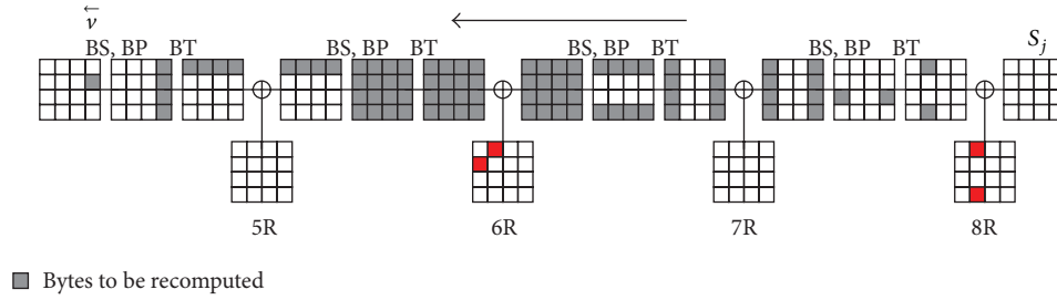
FIGURE 3: Re-computation in the backward direction of Crypton-256.
