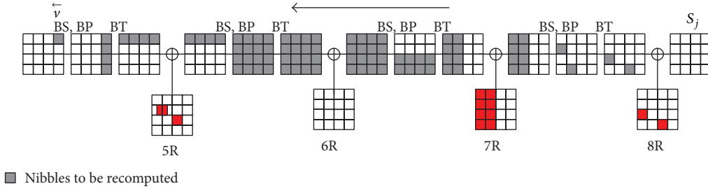
FIGURE 6: Re-computation in the backward direction of mCrypton-128.
