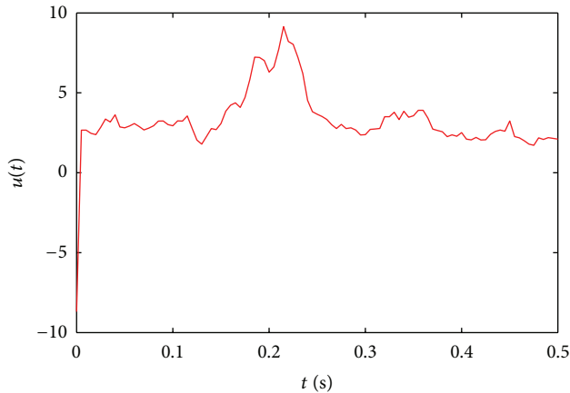
FIGURE 6: The evolution of u(t) .
