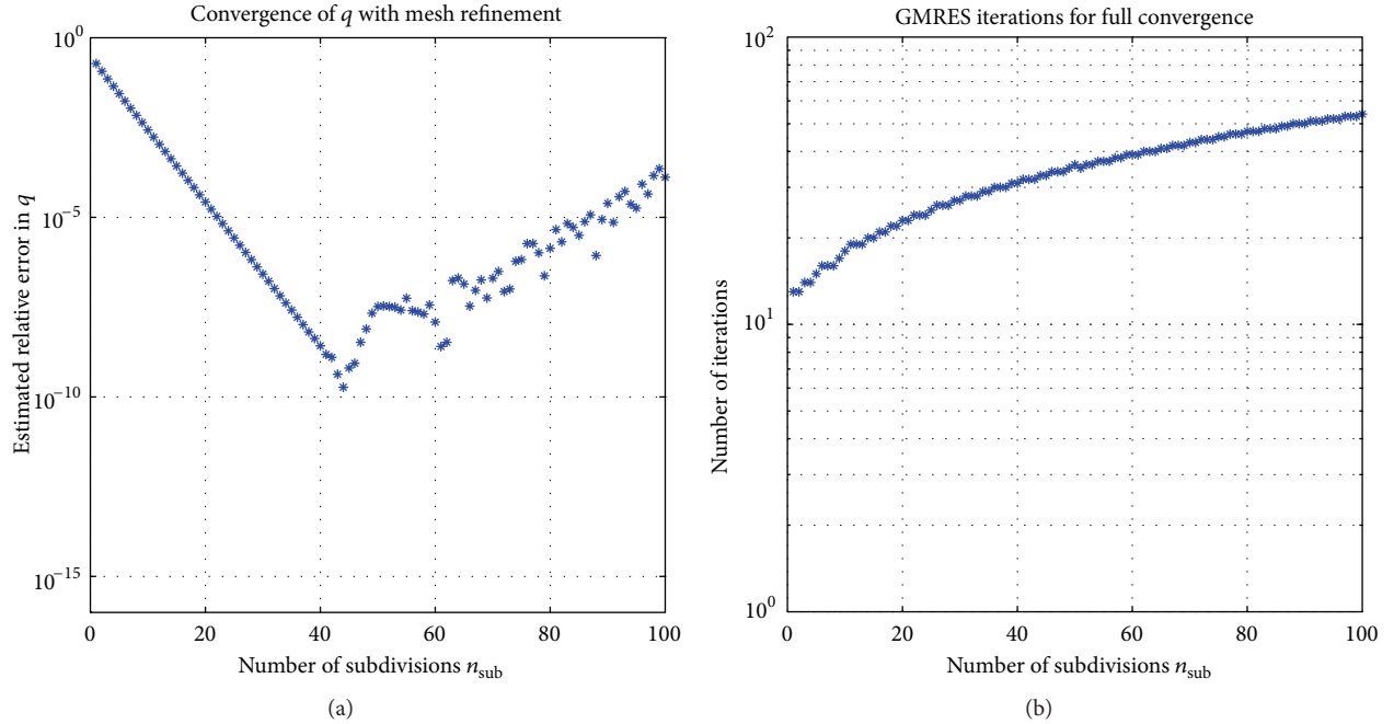
FIGURE 3: Convergence for q of (6) using (8) and the program demo1b.m (a loop of demo1.m ) with \lambda = 0.999 , \theta = \pi/2 , n_{\text{pan}} = 10 , and e_{\text{vec}} = 1 . The reference value is q = 1.1300163213105365 . There are n_p = 160 + 32n_{\text{sub}} unknowns in the main linear system. (a) Convergence with n_{\text{sub}} . (b) The number of iterations needed to meet an estimated relative residual of \epsilon_{\text{mach}} .
