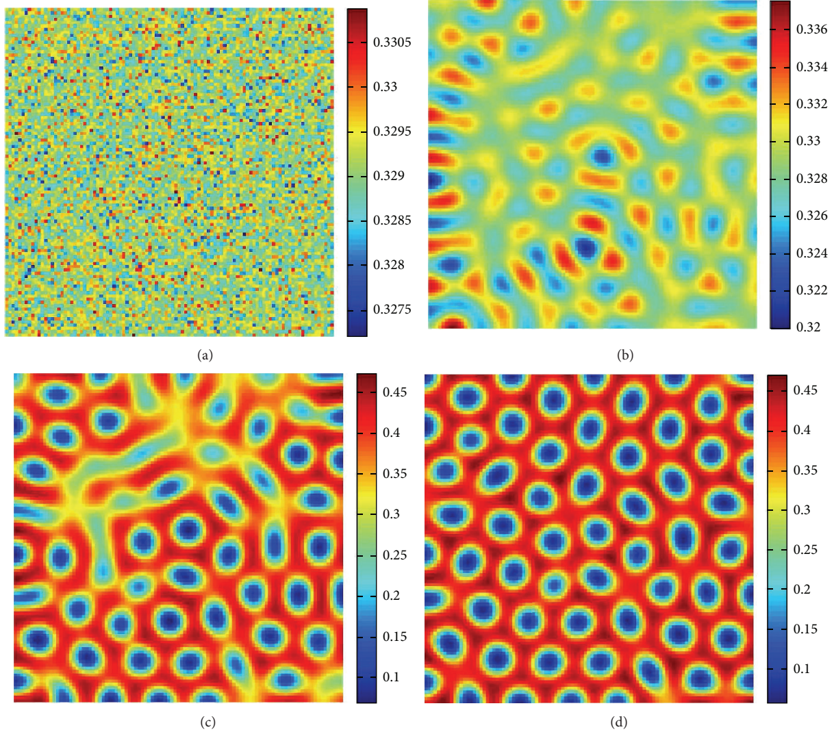
FIGURE 1: Typical Turing patterns of u in model (7) with parameters \alpha = 1, \beta = 0.3, \gamma = 0.3, b = 0.5, c = 0.6, m = 0.6, q = 0.35, s = 1.75, d_1 = 0.015, and d_2 = 1 . Times: (a) 0; (b) 50; (c) 250; (d) 2500.
