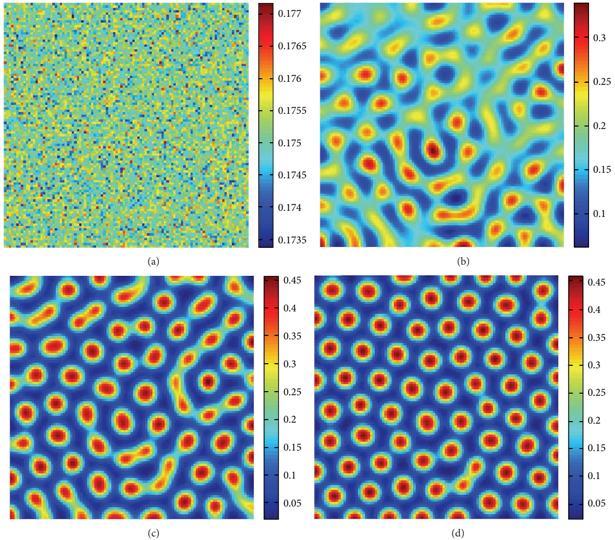
FIGURE 3: Typical Turing patterns of u in model (7) with parameters \alpha = 1, \beta = 0.3, \gamma = 0.3, b = 0.5, c = 0.6, m = 0.6, q = 0.35, s = 3.0, d_1 = 0.015, and d_2 = 1 . Times: (a) 0; (b) 50; (c) 250; (d) 2500.
