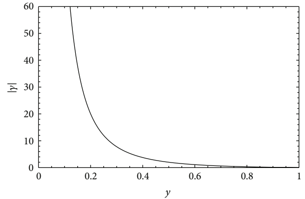
FIGURE 2: Plot of |\gamma(y)| for \epsilon \leq y \leq 1 .
