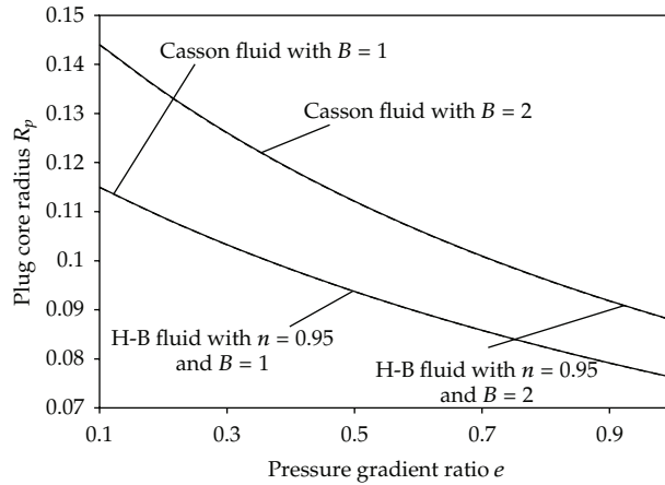
Figure 3: Variation of plug core radius with pressure gradient for H-B and Casson fluids and for different values of body acceleration parameter B with \theta = \delta = 0.1, t = 60^\circ, \phi = 0.7, m = 4, and z = 4 .
