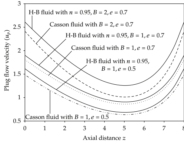
Figure 5: Variation of plug flow velocity with axial distance for H-B and Casson fluids and for different values of B and e with \delta = \theta = 0.1, m = 4, t = 60^\circ, \phi = 0.2, and \omega = 0.5 .
