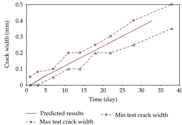
Figure 3: Comparison of predicted crack width over time with published experimental results.
