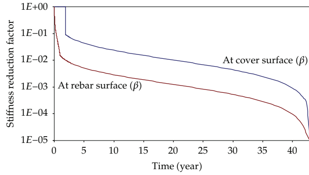
Figure 8: Hoop stiffness reduction factor ( \beta ) at rebar surface and at cover surface with time t .
