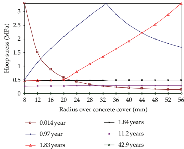
Figure 11: Hoop stress ( \sigma_{\theta} ) varying over concrete cover at various times.
