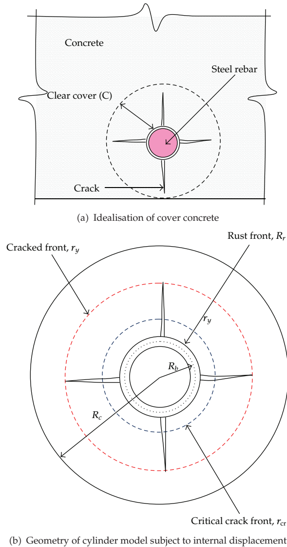
Figure 1: Thick-walled cylinder model for cover concrete cracking evolution due to reinforcement corrosion.
