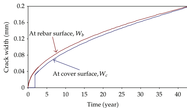
Figure 5: Crack widths at rebar surface ( w_b ) and at cover surface ( w_c ) with time t .
