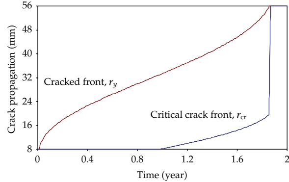
Figure 6: Propagation of cracked front ( r_y ) and critical crack front ( r_{cr} ) with time t .
