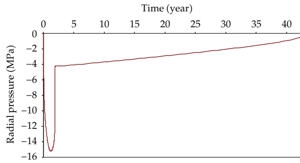
Figure 9: Radial pressure ( \sigma_r ) at rebar surface with time t .
