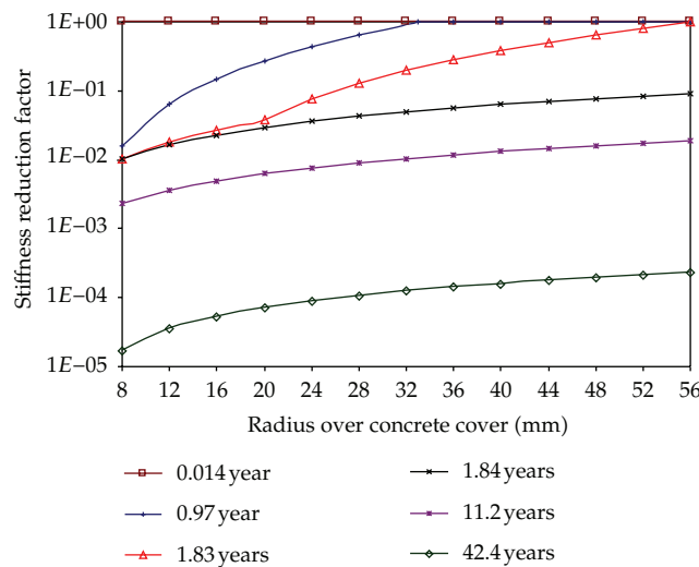
Figure 12: Stiffness reduction factor ( \beta ) varying over concrete cover at various times.
