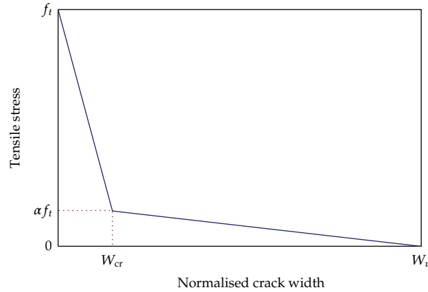
Figure 2: Bilinear softening curve for cohesive cracking in concrete.
