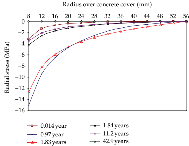
Figure 13: Radial stress ( \sigma_r ) varying over concrete cover at various times.
