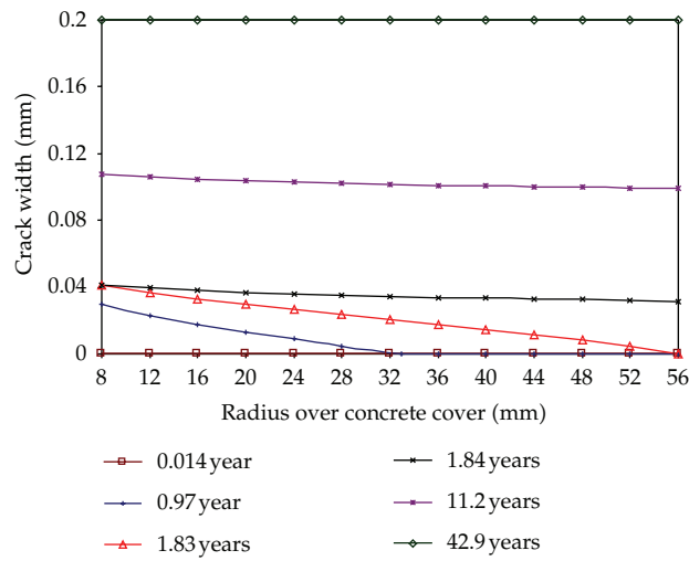
Figure 10: Crack width ( w ) varying over concrete cover at various times.
