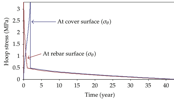
Figure 7: Hoop stress ( \sigma_\theta ) at rebar surface and at cover surface with time t .
