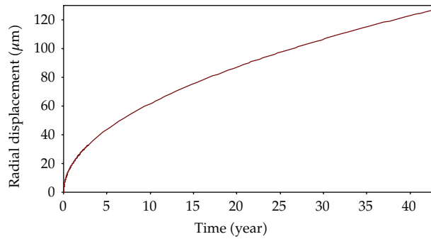
Figure 4: Radial displacement at rebar surface with time t .
