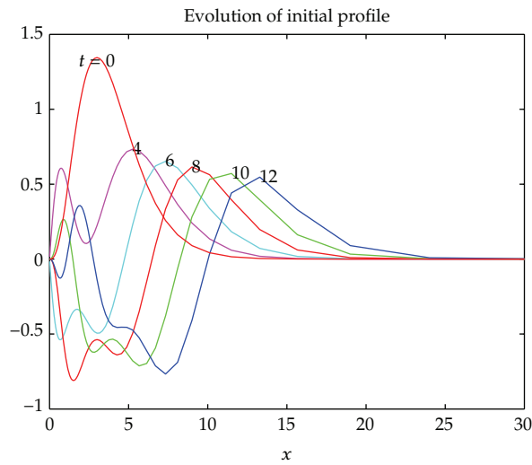
Figure 11: Example 5.2: by quasi-uniform grid.
