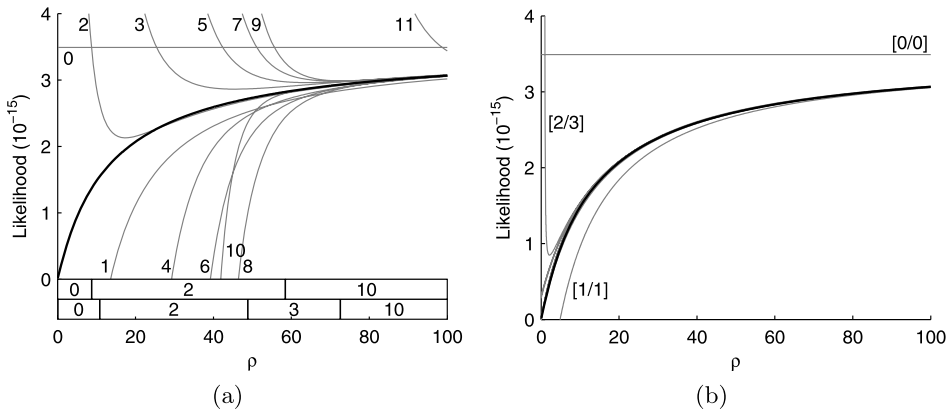
FIG. 2. Likelihood curves for \rho , comparing different levels of truncation, for the sample \mathbf{a} = \mathbf{b} = \mathbf{0} , \mathbf{c} = \begin{pmatrix} 10 & 7 \\ 2 & 1 \end{pmatrix} . A symmetric PIM model with \theta_A = \theta_B = 0.01 is assumed. The true likelihood is shown as a thick black line. Approximate likelihood curves for various levels of truncation, M = 0, 1, \dots, 11 are shown as thinner gray lines. (a) Partial sums q_{PS}^{(M)} , labeled by M . The bottom row of indices records M' , the level of truncation in q_{OTR}^{(11)}(\mathbf{a}, \mathbf{b}, \mathbf{c}) recommended by the OTR. The row above records the actual level of truncation that minimizes the unsigned relative error. (b) Staircase Padé approximants q_{Padé}^{[U/V]} , some labeled by [U/V] . To the naked eye, q_{Padé}^{[U/V]} for most [U/V] are indistinguishable from the true likelihood curve.
