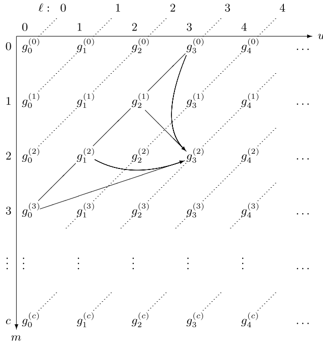
FIG. 1. Computation of g_u^{(m)} for each m = 0, \dots, c and u = 0, 1, \dots . When m > 0 , the term g_u^{(m)} residing on level \ell = m + u is determined by up to four entries on level \ell - 2 . This is illustrated for the example g_3^{(2)} .
