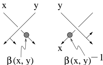
Fig. 5. The beads interpretation of the invariant
