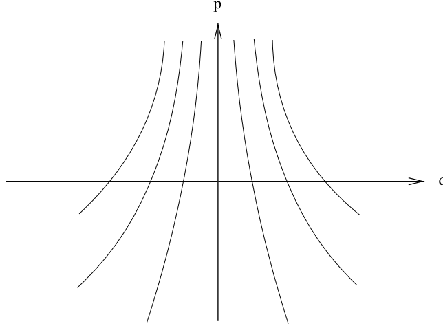
Figure 2. The monoid of Example 6 is a local symplectic groupoid if restricted to a neighborhood of the units.
