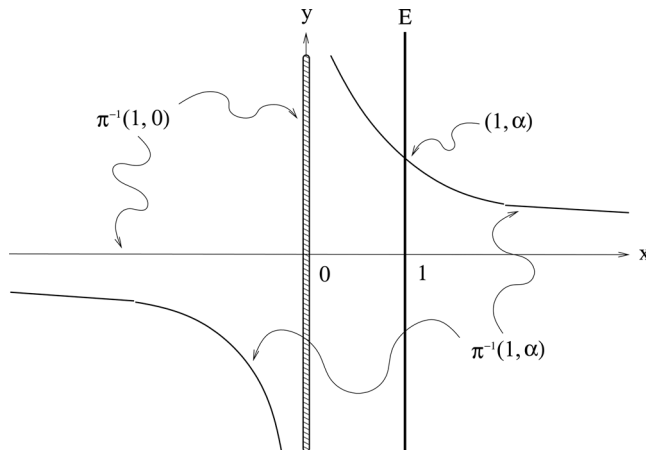
Figure 1. The source (and target) fibre \pi^{-1}(1, 0) is singular.
