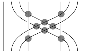
Figure 4: (\sigma'_1 \xi) \cdot (\bar{\xi}) , with relevant crossings shaded
