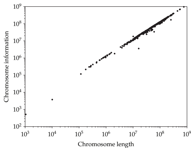
Figure 7: Chromosome length L_i^{\text{chrom}} versus its information content I_i^{\text{chrom},8} , i = 1, \dots, 463 , n = 8 .
