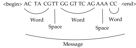
Figure 2: Example of a message when considering n = 2 , \{TT, AA\} \equiv "spaces", \{TC, TA, TG, CT, CC, CA, CG, AT, AC, AG, GT, GC, GA, GG\} \equiv "word characters." Multiple consecutive spaces are considered as a single space.
