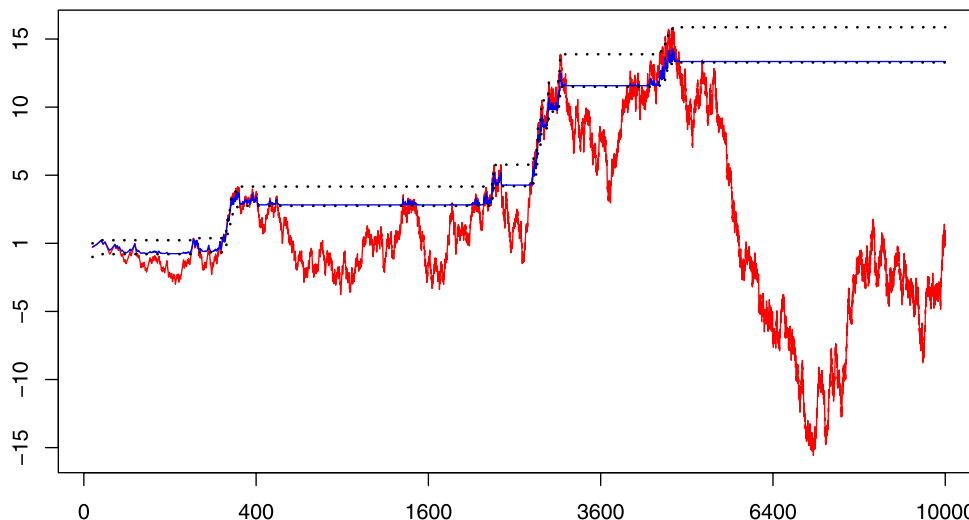
FIG. 2. The red line is a realization over 10,000 trials of the likelihood ratio for testing \theta = 1/2 against \theta = 3/4 . The horizontal axis gives the number of observations so far. The vertical axis is logarithmic and is labeled by powers of 10. The likelihood ratio varies wildly, up to 10^{15} and down to 10^{-15} . Were the sequence continued indefinitely, it would be unbounded in both directions.
