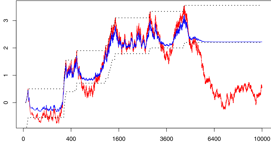
FIG. 3. A realization over 10,000 trials of the likelihood ratio for testing \theta = 1/2 against the probability distribution Q obtained by averaging P_\theta with respect to the uniform distribution for \theta . The vertical axis is again logarithmic. As in Figure 2, the oscillations would be unbounded if trials continued indefinitely.
