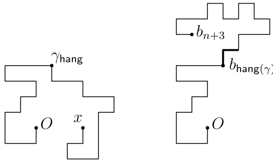
FIG. 5. Left: A self-avoiding walk \gamma \in F_j . Right: A walk b \in \Phi(\gamma) . The point b_{\text{hang}(\gamma)} is the (j + 1) st z -renewal point of b ; it is followed by the edges e_1, e_2 (in bold), then by a half-space walk of length n - \text{hang} + 1 .
