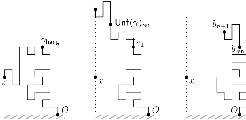
FIG. 3. Left: A walk \gamma \in \text{SAHSW}_n ending at x . Middle: The unfolding of \gamma , \text{Unf}(\gamma) , and its last renewal point \text{Unf}(\gamma)_{\text{ren}} . Notice the bold edge e_1 added between \gamma^1 and the reflection of \gamma^2 . Right: A walk b \in \Phi(\gamma) . Its last renewal point is b_{\text{ren}} ; b[0, \text{ren}] is a bridge and b[\text{ren}, n + 1] is equal up to translation to \text{Unf}(\gamma)[\text{ren}, n + 1] (bold). The choice of b[0, \text{ren}] may be such that \pi_1(b_{n+1}) \neq \pi_1(x) .
