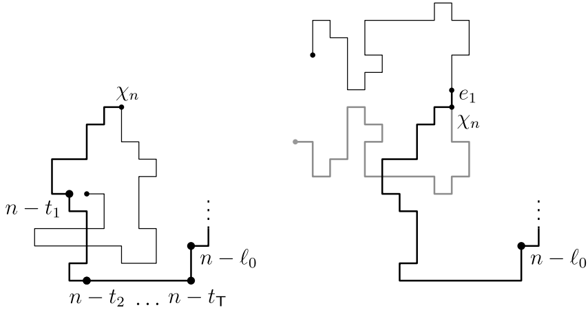
FIG. 7. Left: The final portion of \chi in bold, and a walk contained in C_1 and in A_1 but not in A_2 . Right: A walk \gamma \in W \setminus A (gray) may be reflected and added to \chi^{\ell_0} (black) to create a walk starting with \chi^{\ell_0} , with hanging point different from \chi_n . When concatenating \mathcal{R}_{\chi_n}(\gamma) to \chi^{\ell_0} , an extra vertical edge is added in to ensure nonintersection, and the last edge is deleted to preserve length n .
