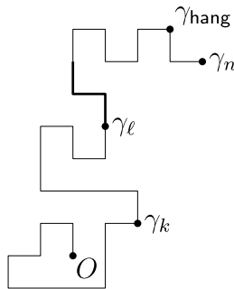
FIG. 2. A walk \gamma with a renewal point \gamma_k , a z-renewal point \gamma_\ell and hanging point \gamma_{\text{hang}} . The bold structure beyond the point \gamma_\ell helps to ensure that \ell is a z-renewal time. Both \gamma[k, \ell] and \gamma[k, \text{hang}] are bridges.
