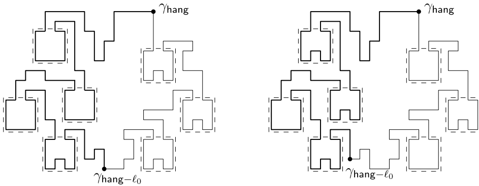
FIG. 6. In a closing walk the \ell_0 steps up to the hanging point form a good walk (bold). By exchanging type I and II patterns between the bold and regular part of the walk in a way that increases by order n^{1/2} the number of type II patterns in the bold part, we may effectively shorten the good part by an amount of this order.
