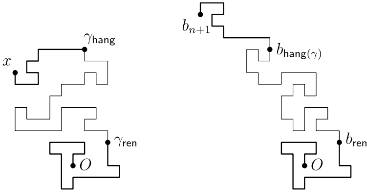
FIG. 4. Left: A walk \gamma \in E_M(x) . Right: A walk b \in \Phi(\gamma) . The first and last parts of b (bold) are the same as those of \gamma (up to translation and reflection). Its middle part is a bridge with appropriate length and e_1 -displacement.
