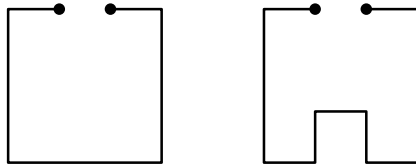
FIG. 1. An example of type I and II patterns for d = 2 .
