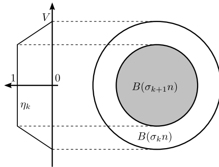
FIG. 1. Illustration of both the balls B(\sigma_k n) and B(\sigma_{k+1}n) and the corresponding cut-off function \eta_k .
