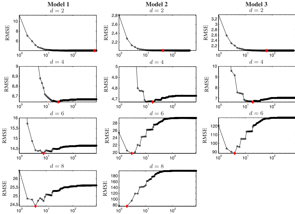
FIG. 5. Root mean squared error (RMSE) for out-of-sample predictions of simulations with different dimensions d . The x -axis in each figure corresponds to the number of partitions made by IRP, that is, the curves show how the RMSE of test data varies as the IRP algorithm progresses. Model 1 uses the function y_i = (\sum_j x_{ij}^2) + \mathcal{N}(0, 4d^2) with x_{ij} \sim \mathcal{U}[0, 5] . Model 2 uses the function y_i = (\prod_j x_{ij}) + \mathcal{N}(0, d^2) with x_{ij} \sim \mathcal{U}[0, 3] . Model 3 uses the function y_i = 2\sum_j x_{ij} + \mathcal{N}(0, d^2) with x_{ij} \sim \mathcal{U}[0, 2] . Fifty simulations were run with 12,000 training and 3,000 testing points. Only the first 750 partitions of the paths are displayed in order to make the RMSE of the earlier IRP iterations visually clearer.
