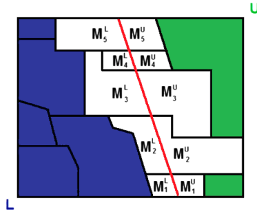
FIG. 8. Illustration of the proof of Theorem 2. Black lines separate blocks. The diagonal red line through the center demonstrates a cut of Algorithm 1. \mathcal{L} is the union of blue blocks below the cut and \mathcal{U} is the union of green blocks above the cut. White blocks are blocks that are potentially split by Algorithm 1. These blocks are split into M_1^L, \dots, M_5^L below the cut and M_1^U, \dots, M_5^U above the cut. In the proof, M_i = M_i^L \cup M_i^U for all i = 1, \dots, 5 . The proof shows, for example, that if the algorithm splits M_1 into M_1^L and M_1^U according to the defined cut in (5), then there must be no isotonicity violation when creating blocks from M_1^L and M_1^U . However, since M_1 is assumed to be a block, there must exist an isotonicity violation between M_1^L and M_1^U , providing a contradiction.
