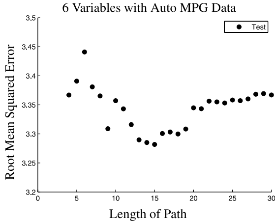
FIG. 6. Root mean squared error (RMSE) for auto data with six variables using IRP illustrates that overfitting occurs after 15 iterations of IRP, that is, RMSE decreases until 15 partitions are made, after which RMSE begins to increase. The figure displays only the first 30 partitions so that the U-shape is clear.
