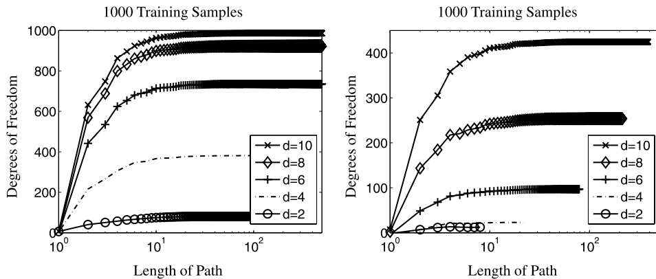
FIG. 3. Evolution of degrees of freedom for IRP as model complexity increases. Both models use y_i = \sum_j x_{ij}^2 + \mathcal{N}(0, 10) . Simulation (left) uses x_{ij} \sim \mathcal{U}[1, 2] and simulation (right) uses x_{ij} \in \{0, 1, 2\} with probabilities \{1/3, 1/3, 1/3\} . Each path is the mean over 50 trials with 1,000 training samples.
