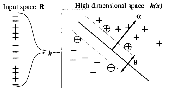
FIG. 6. The maximal margins classification method. In this example, the raw data point x is an element of \mathbb{R} , but in that space the positive and negative examples are not linearly separable. The raw input is mapped to a point in a high-dimensional space (here \mathbb{R}^2 ) by a fixed nonlinear transformation \mathbf{h} . In the high-dimensional space, the classes are linearly separable. The vector \alpha is chosen to maximize the minimal margin \theta . The circled instances are the support vectors; Vapnik shows that \alpha can always be written as a linear combination of the support vectors.
