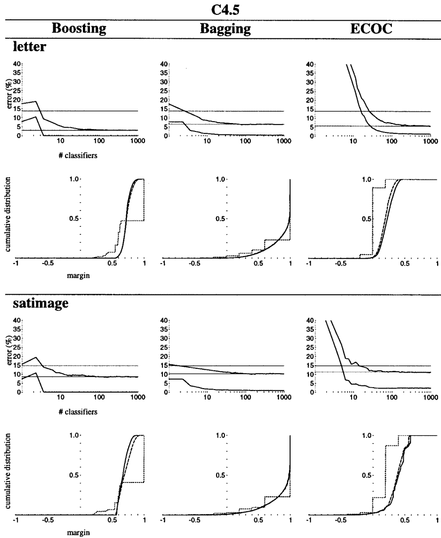
FIG. 4. Error curves and margin distribution graphs for three voting methods (bagging, boosting and ECOC) using C4.5 as the base learning algorithm. Results are given for the letter, satimage and vehicle datasets. (See caption under Figure 1 for an explanation of these curves.)
