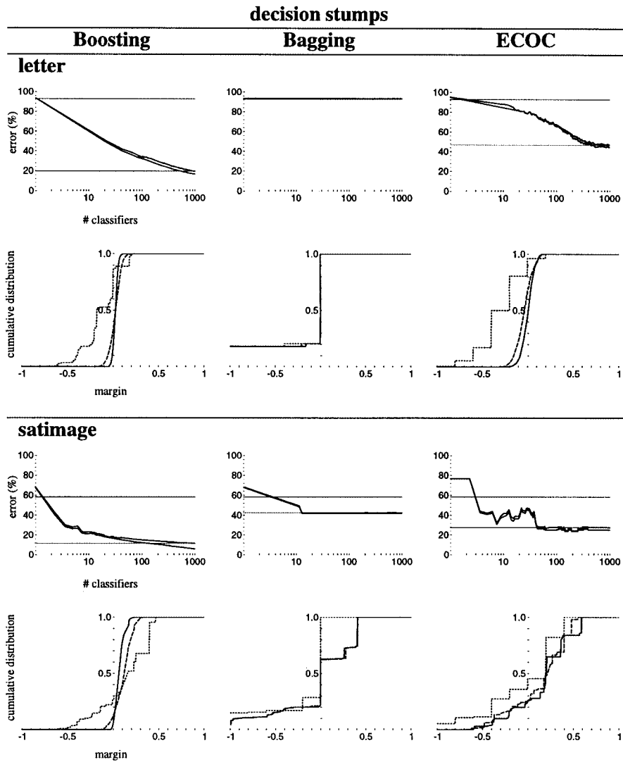
FIG. 5. Error curves and margin distribution graphs for three voting methods (bagging, boosting and ECOC) using decision stumps as the base learning algorithm. Results are given for the letter, satimage and vehicle datasets. (See caption under Figure 1 for an explanation of these curves.)
