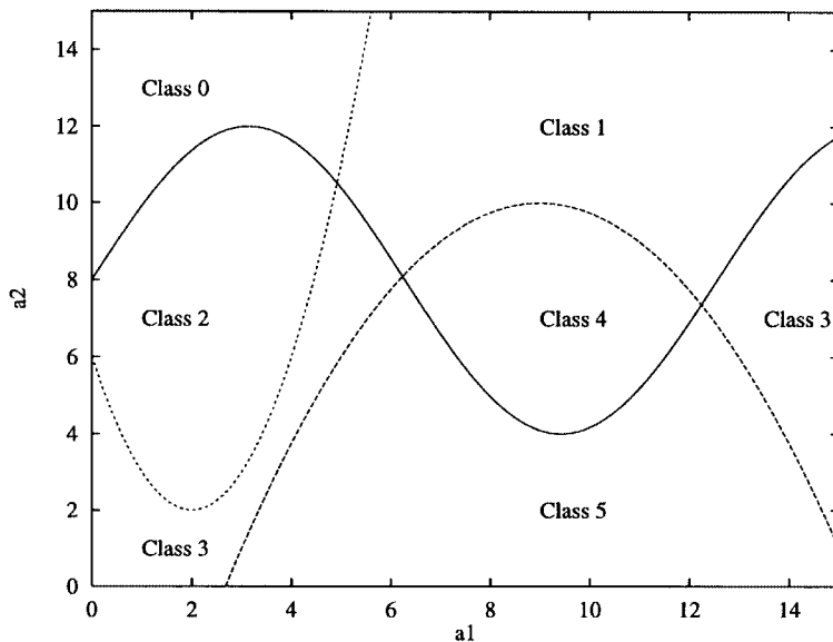
FIG. 7. The 2-dimension, 6-class classification problem defined by Kong and Dietterich [26] on the region [0, 15] \times [0, 15] .
