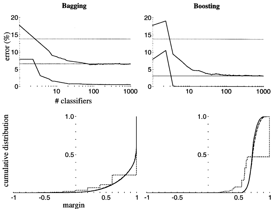
FIG. 1. Error curves and margin distribution graphs for bagging and boosting C4.5 on the letter dataset. Learning curves are shown directly above corresponding margin distribution graphs. Each learning curve figure shows the training and test error curves (lower and upper curves, respectively) of the combined classifier as a function of the number of classifiers combined. Horizontal lines indicate the test error rate of the base classifier as well as the test error of the final combined classifier. The margin distribution graphs show the cumulative distribution of margins of the training instances after 5, 100 and 1000 iterations, indicated by short-dashed, long-dashed (mostly hidden) and solid curves, respectively.
